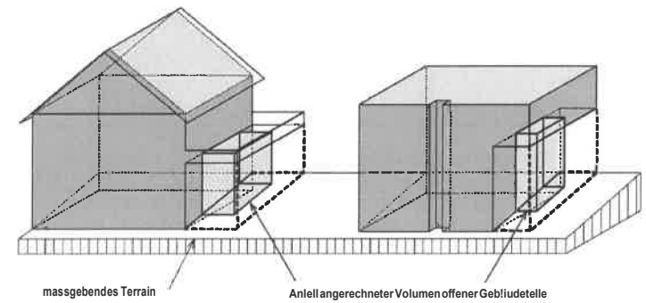
Figur 7.3 Baumannsziffer
